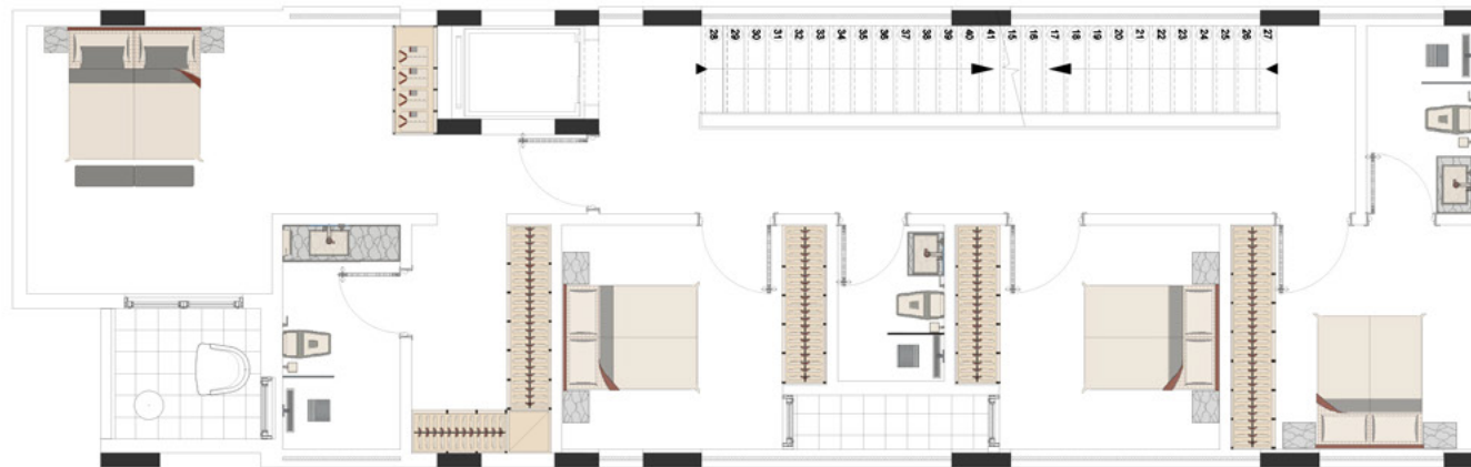
FIRST FLOOR
