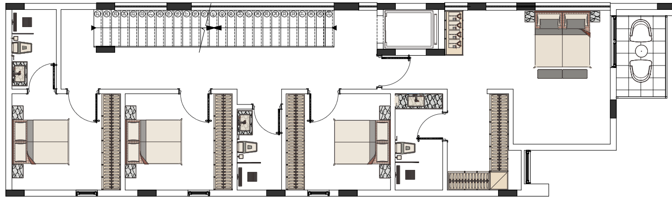
FIRST FLOOR
