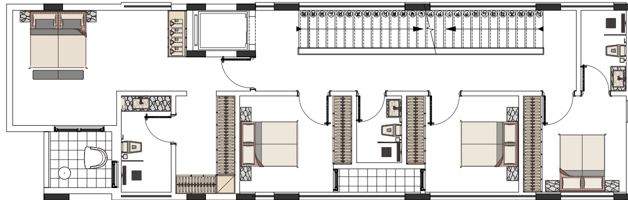
FIRST FLOOR
